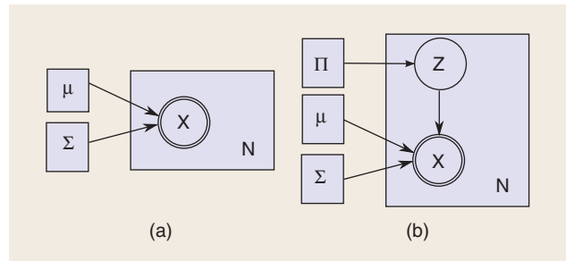
[FIG5] Graphical models (a) for a single Gaussian component, (b) for a Gaussian mixture model.
