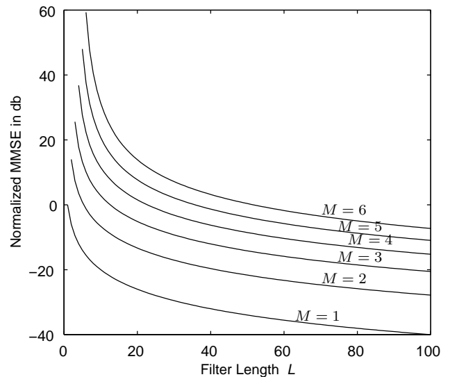
Figure 1: Normalized MMSE in db for polynomial orders M-1 = 0, \dots, 5 and filter lengths L = M, \dots, 100 .
